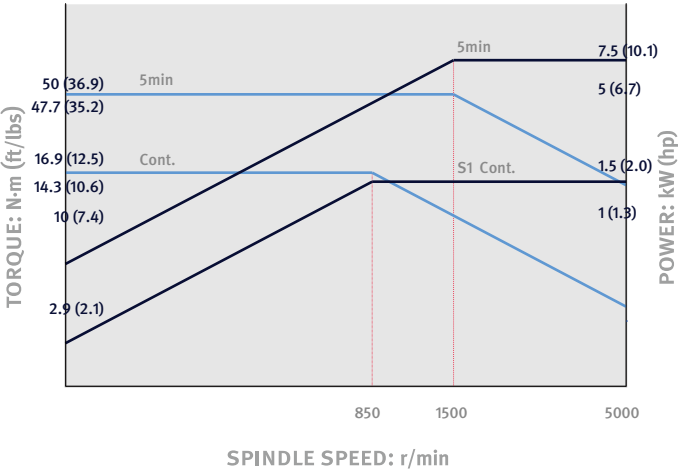
Rotary Tool_ Lynx 2600Y/SY 16st.
