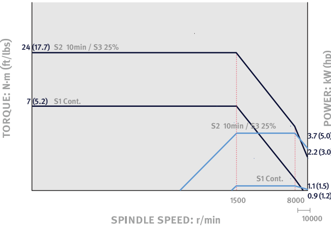
Rotary Tool_ Lynx 2100LY / LSY OPTION
