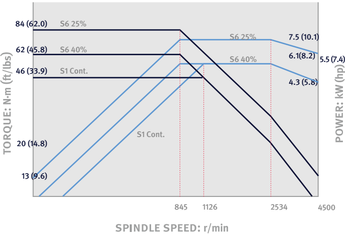
Sub-Spindle_ Lynx 2600Y/SY
