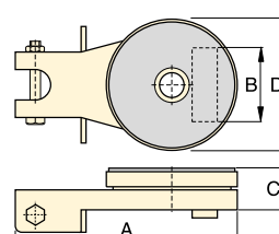
ES10, ES15, ES30 Placa giratoria
